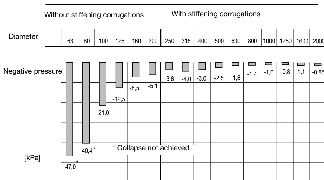
Collapsing pressure
